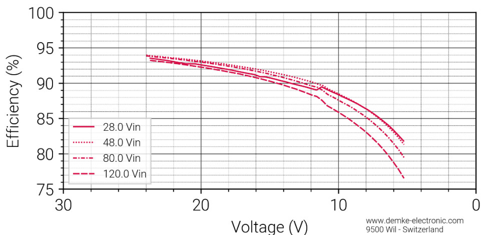
Figure 3 Efficiency in the constant current range of the DC-Transformer 154DH-24-ON
