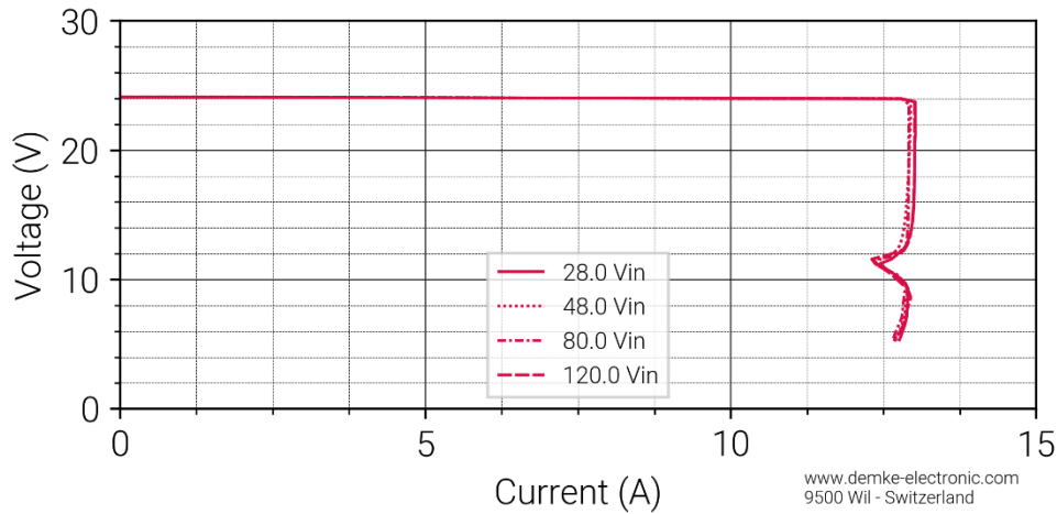
Figure 1 Voltage against current of the DC-Transformer 154DH-24-ON
