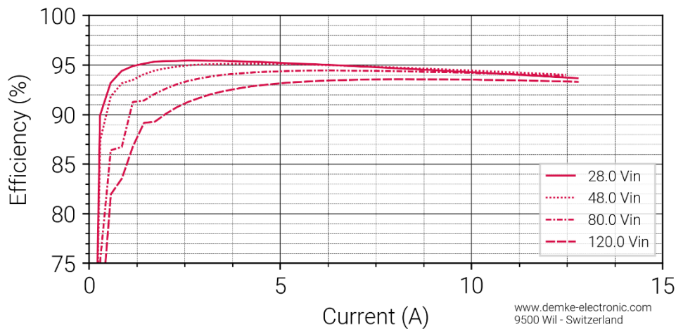
Figure 2 Efficiency in the constant voltage range of the DC-Transformer 154DH-24-ON
