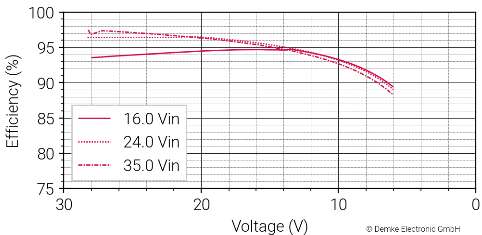
Figure 3 Efficiency in the constant current range of the DC-Transformer 257E-28-SD
