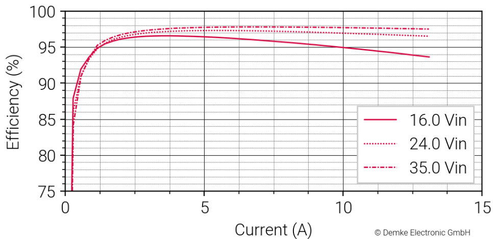
Figure 2 Efficiency in the constant voltage range of the DC-Transformer 257E-28-SD
