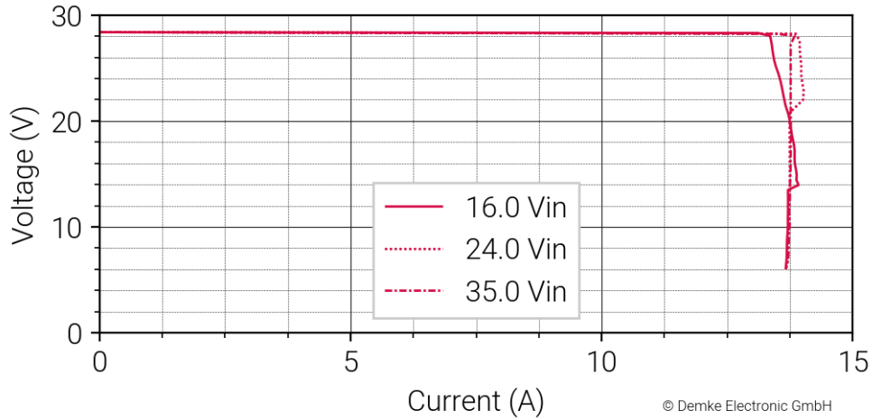
Figure 1 Voltage against current of the DC-Transformer 257E-28-SD
