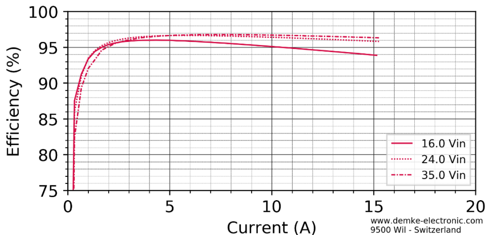
Figure 2 Efficiency in the constant voltage range of the DC-Transformer 257E-24-SD
