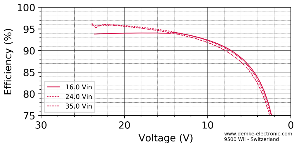
Figure 3 Efficiency in the constant current range of the DC-Transformer 257E-24-SD
