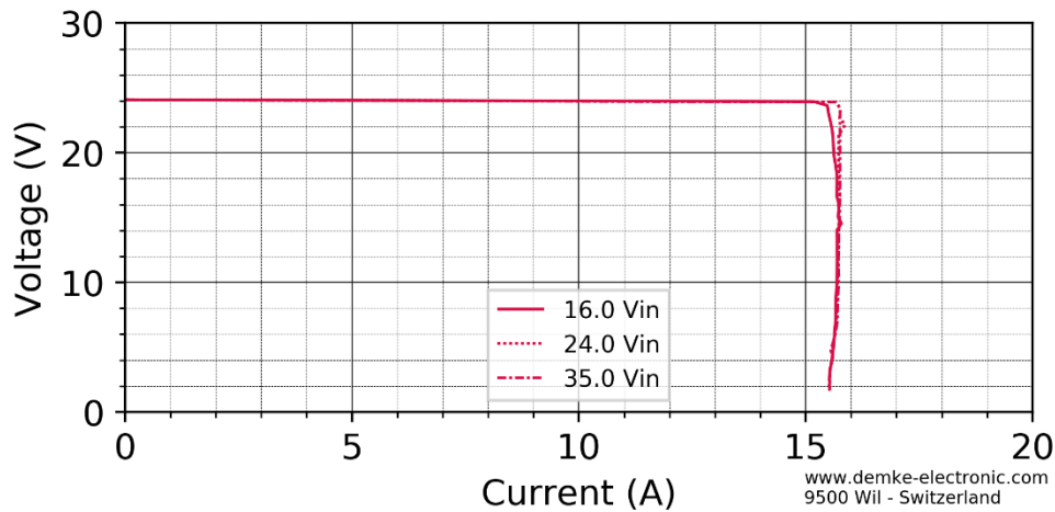
Figure 1 Voltage against current of the DC-Transformer 257E-24-SD
