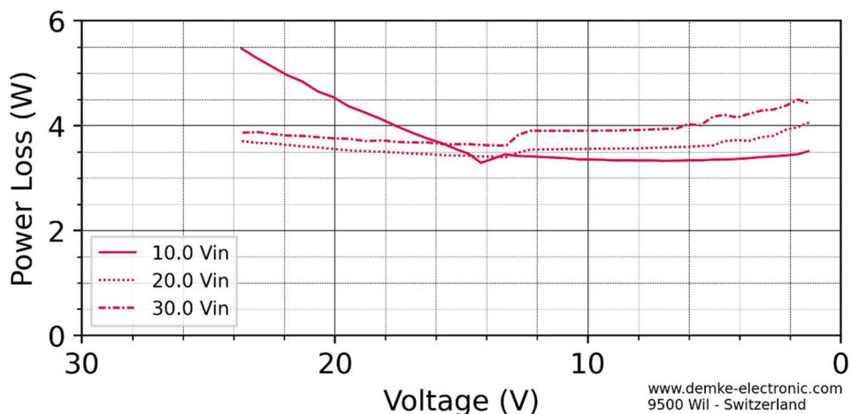
Figure 5: Power Loss over voltage of the DC-Transformer 331-24-SD
