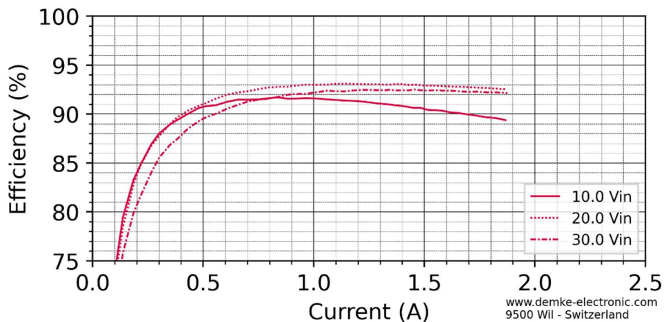
Figure 2 Efficiency in the constant voltage range of the DC-Transformer 331-24-SD
