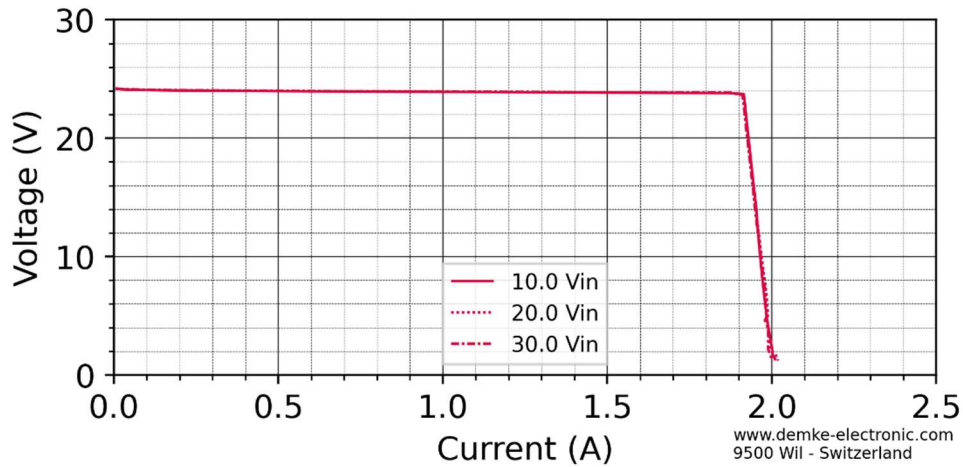
Figure 1 Voltage against current of the DC-Transformer
