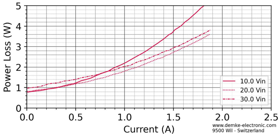
Figure 4: Power Loss over current of the DC-Transformer 331-24-SD
