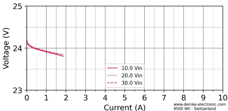
Figure 6: Voltage in CV-mode of the DC-Transformer 331-24-SD
