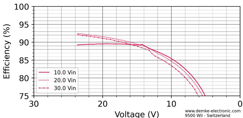
Figure 3 Efficiency in the constant current range of the DC-Transformer 331-24-SD
