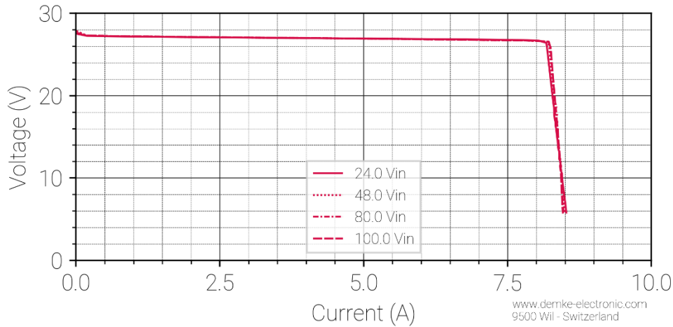
Figure 1 Voltage against current of the DC-Transformer 365DH-27-SD
