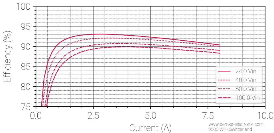
Figure 2 Efficiency in the constant voltage range of the DC-Transformer 365DH-27-SD
