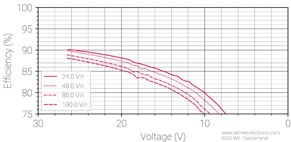
Figure 3 Efficiency in the constant current range of the DC-Transformer 365DH-27-SD
